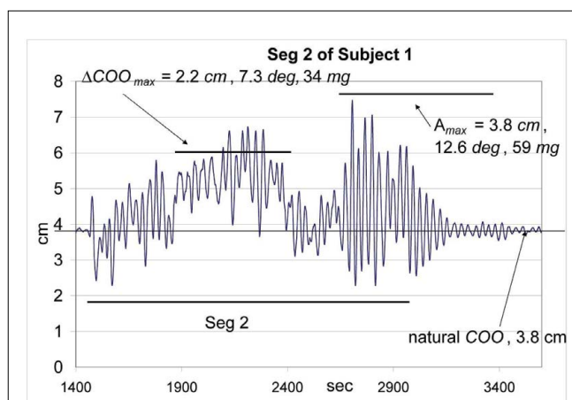
Figure 7: Focus on Seg 2 of Figure 6 data. Figure 6 shows the results of three consecutive experiments with Subject 1 under the pendulum. Figure 7 focuses on Seg 2 data of Figure 6. The duration of Seg 2 is about 1,700 sec (28 min), and during that time, the COO shifts 2.2 cm away from the natural COO. This corresponds to 7.3 deg of rotation, and based on the \kappa of the monofilament fiber, would require a force that is equivalent to 34 mg.
