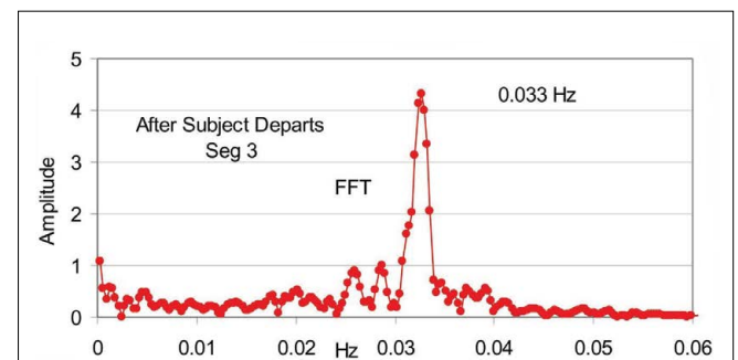
Figure 15: FFT analysis of the post-Seg 3 oscillations in Figure 14. To be compared to the FFT analysis of data in Figure 3 in which no Subject was present. Figure 15 shows a frequency peak at 0.033 Hz, which corresponds to the 0.034 Hz frequency obtained in the absence of a Subject. The major difference is that Figure 15 shows many new frequencies that are absent from Figure 3. Figure 16 shows these additional frequencies in greater detail.
