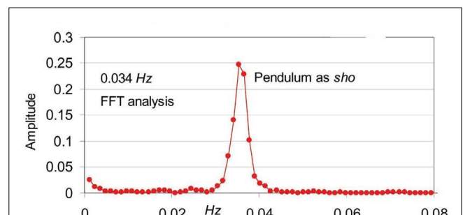
Figure 4: FFT of natural oscillations of the pendulum. FFT analysis of the data in Figure 3 using SigView as described in Materials and Methods. It shows that the natural frequency of the pendulum, in the absence of a Subject, is about 0.034 Hz , which is equivalent to a period of 29.4 sec .
