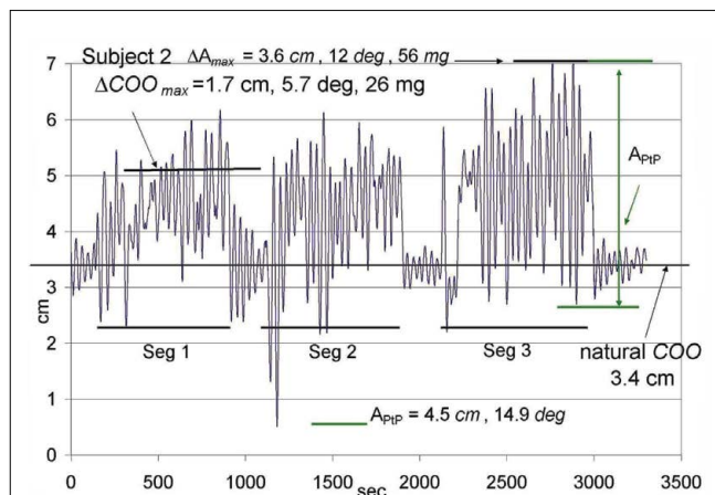
Figure 20: A three-Seg experiment performed with Subject 2. The initial seconds of the experiment are oscillations prior to Subject 2 being seated under the pendulum. Seg 1 is a period of time during which Subject 2 is seated under the pendulum, as are Seg 2 and Seg 3, respectively. When the Subject is present, the amplitudes of the oscillations and the Center of Oscillation (COO) of the pendulum both change dramatically, with the maximum \Delta\text{COO} expressed as cm, deg of rotation, and mg of force required to drive the rotation. A_{\text{max}} is the maximum amplitude of the displacement from the natural COO expressed as cm, deg of rotation, and mg of force. The vertical green arrow is the A_{\text{PtP}} , which is the largest peak-to-peak amplitude observed during the experiment, expressed as cm and deg of rotation. The results with Subject 2 can be compared with Subject 1 (Figure 6) and with Subject 3 (Figure 21).
