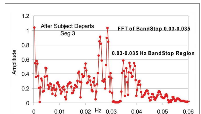
Figure 16: FFT analysis of 0.03-0.035 Hz BandStop of Figure 14 oscillations. The 0.03-0.035 Hz frequency component was removed from the oscillation signal of Figure 14. Figure 16 shows the FFT analysis of the remaining signal components. Many frequency components remain, as described in Results.
