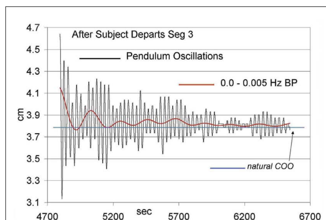
Figure 17: Overlay of 0.0-0.005 Hz BandPass component onto the post-Seg 3 oscillation signal from Figure 15.
