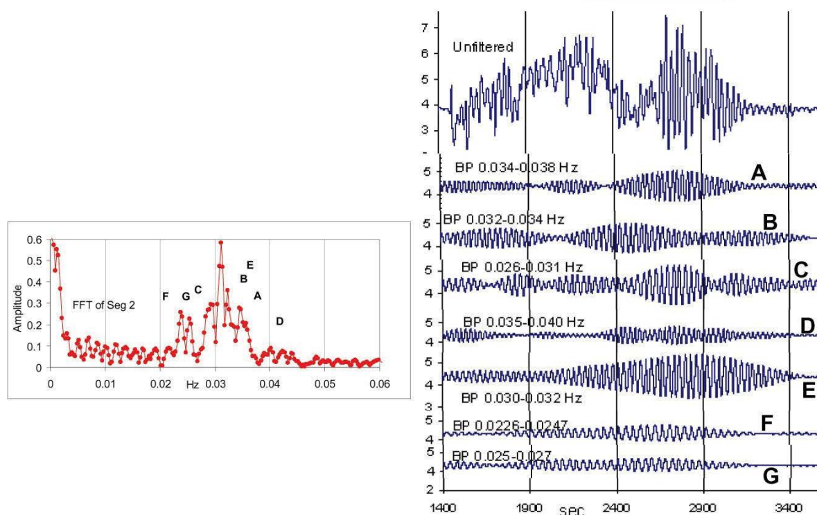
Figure 10: Frequency components that contribute to the oscillation profile of Seg 2. The right top panel shows oscillation data of Seg 2, including several min after the Subject left the pendulum. The FFT analysis of these data is shown in the left panel. Each of the A-G frequency peaks corresponds to a particular frequency range that is responsible for that peak. The contribution of each peak is assessed by applying a BandPass filter to the frequency range that is defined by the lowest amplitudes above and below each peak. For curves A-G, what is represented is the BandPass (BP) profile that represents the frequency contribution of that particular BP component to the top panel data, e.g., curve A is what is obtained by applying a 0.034-0.038 Hz BandPass filter to the top panel data.
